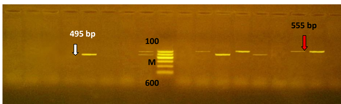
Fig (2) C. jejuni toxins showed at 555 bp for CdtC and at 495 bp for CdtB. Lane M: 100 bp – 600 bp ladder; Lane: 2, 4, 7 C. jejuni CdtC at 555bp Lane: 1, 5, 6, and 11 C. jejuni CdtB at 495b.
