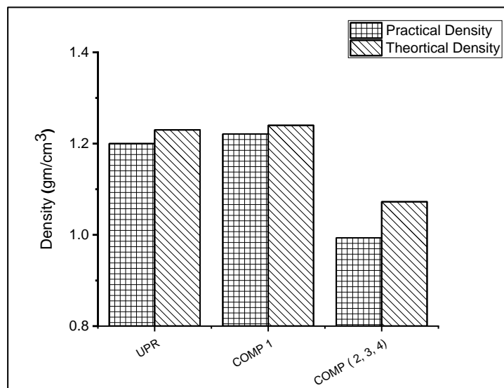
Fig. (5) Practical vs theoretical density.
